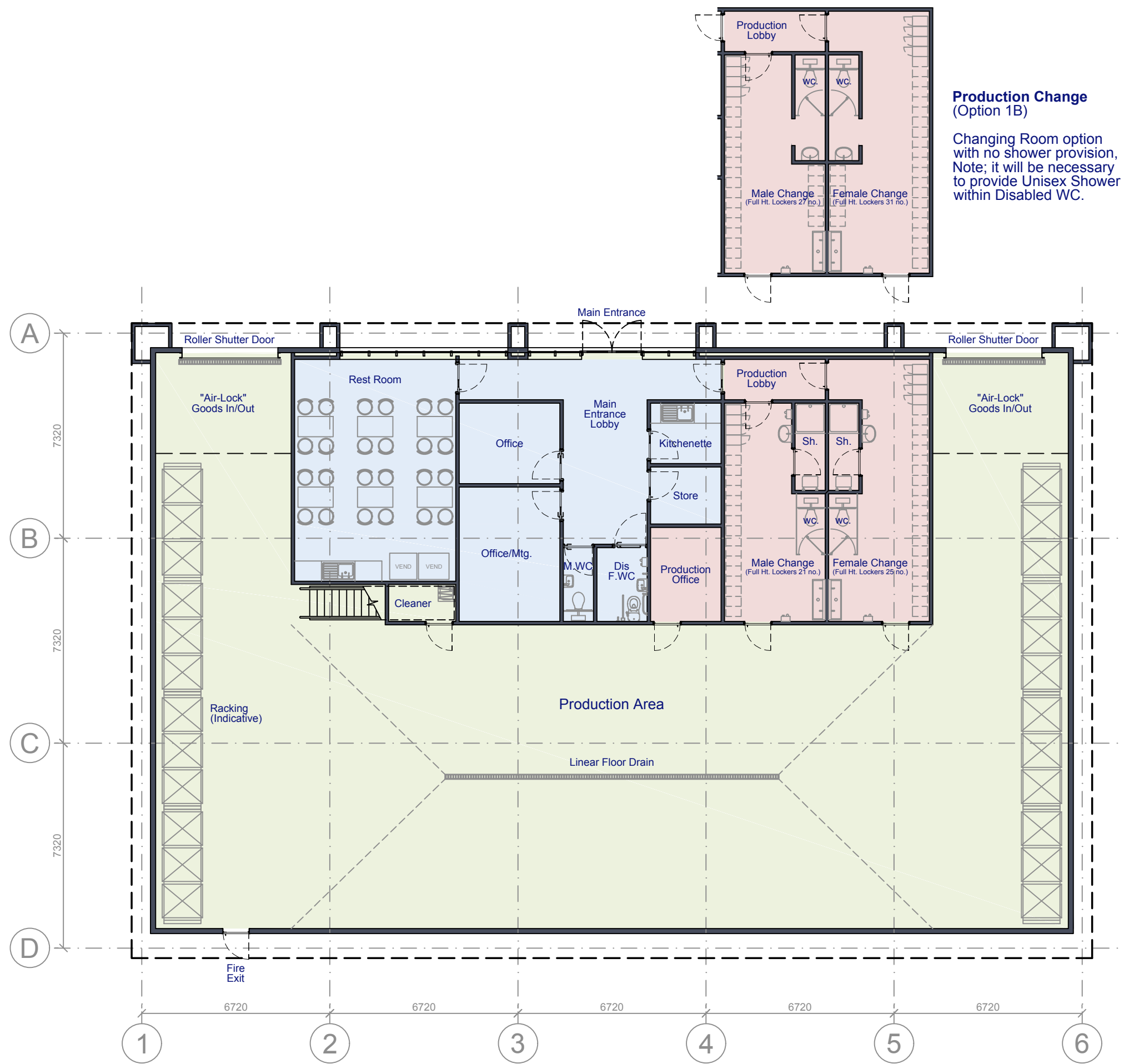
Ground Floor Layout
